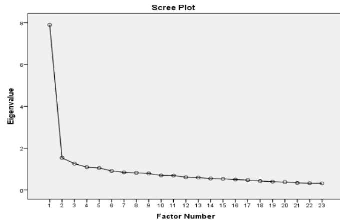
Figure 1. Plot Results of exploratory factor analysis
